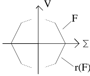
FIGURE 1. Thurston norm ball on H_2(D_M, \partial D_M; \mathbb{R}) = \mathbb{R} \cdot \Sigma \oplus V .
