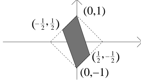
FIGURE 9. Twisted Alexander norm ball for Dunfield's link
