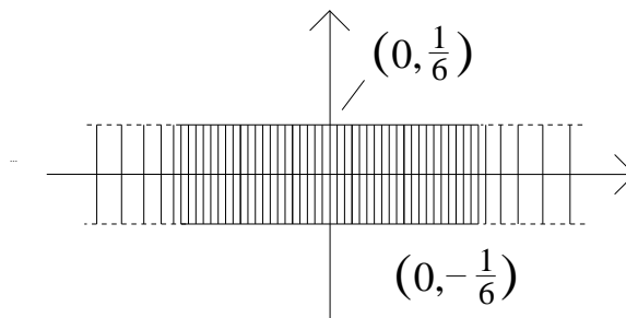
FIGURE 6. Thurston norm ball of L .
